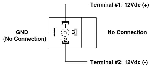
Figure 16: Solenoid DIN Connector Connection
