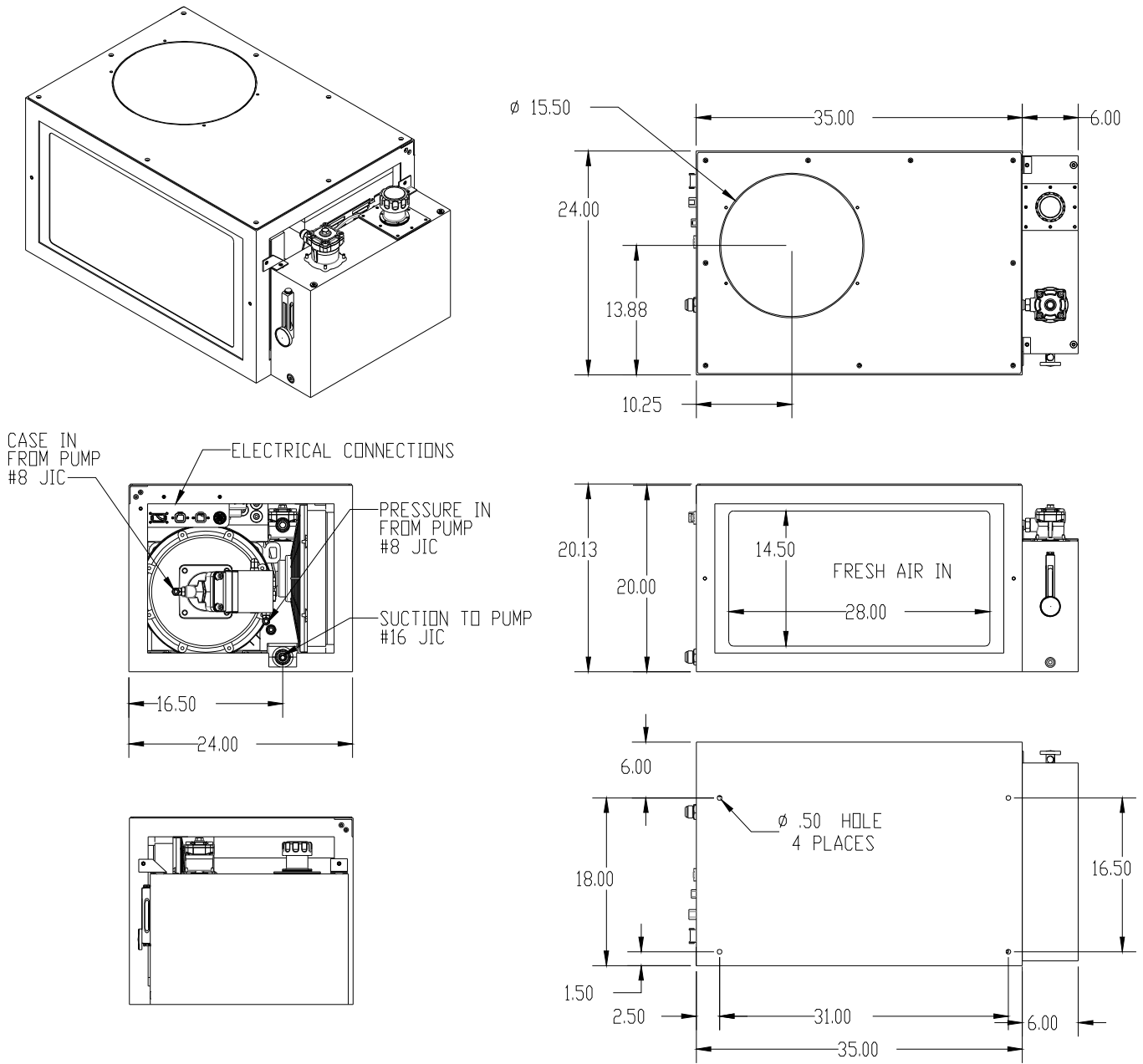
Figure 2: Generator Tray Dimension Drawing (MPC 30KW)
