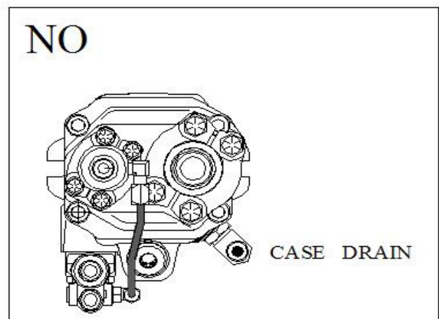
Figure 9: Pump Case Drain Orientation
