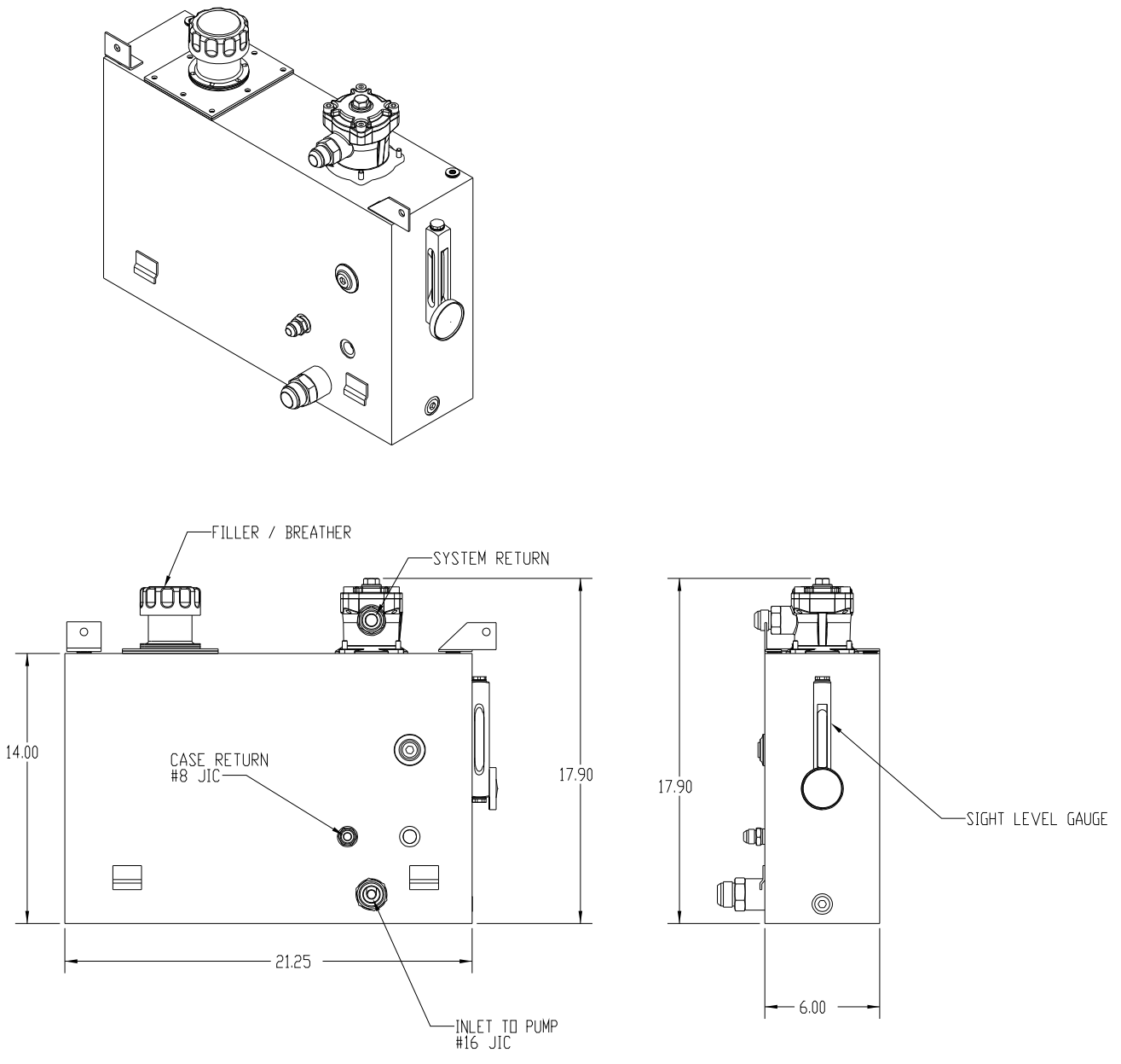
Figure 3: Reservoir Dimension Drawing
