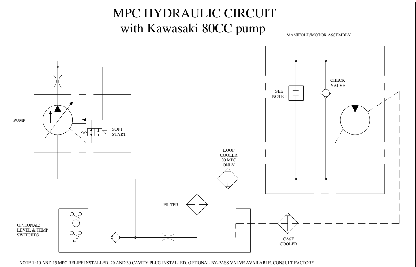
Figure 13: Hydraulic Circuit Diagram with Kawasaki 80cc Pump
