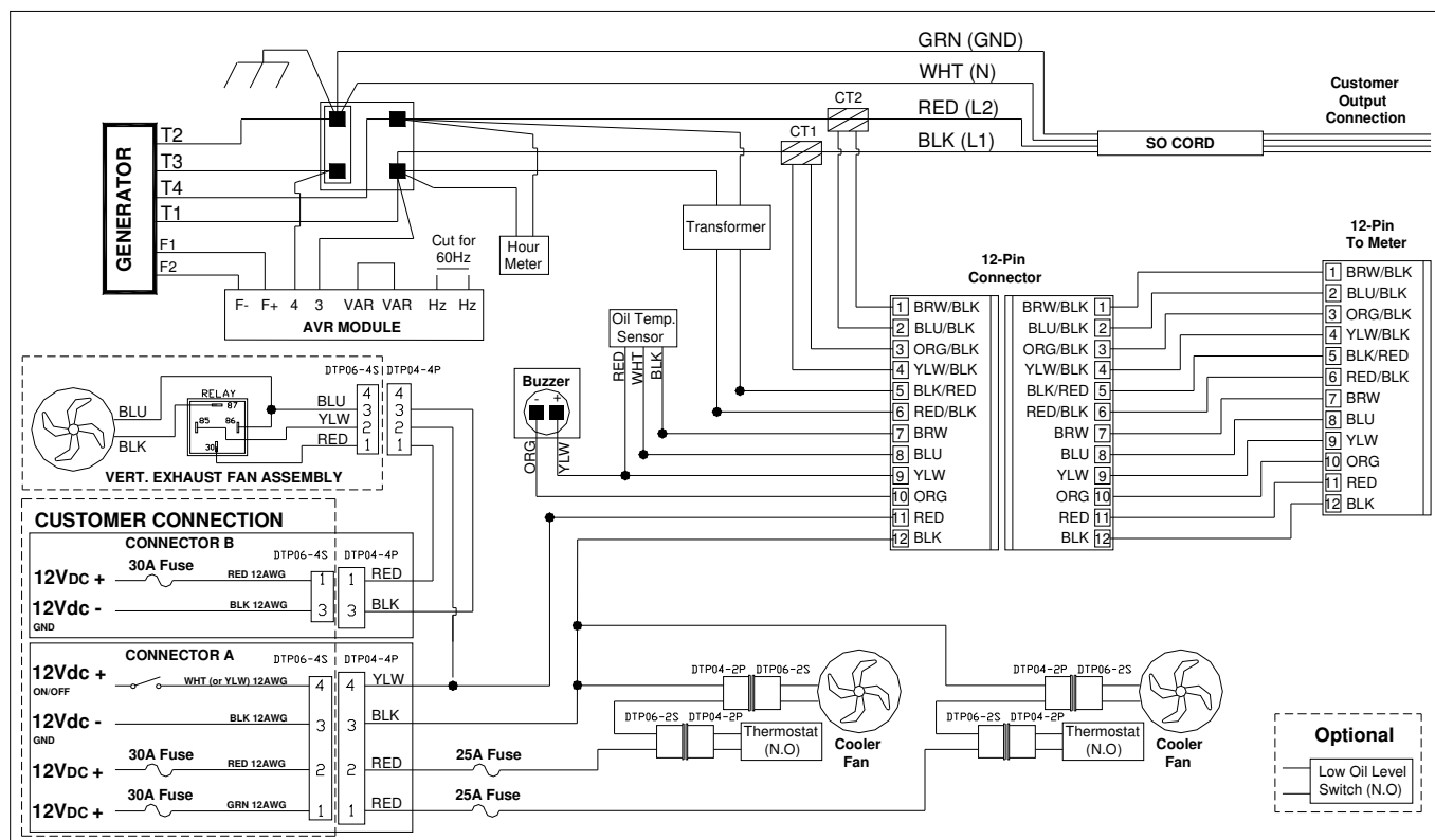
Figure 18: 30KW MPC Electrical Circuit Diagram for 120/240 1ph
