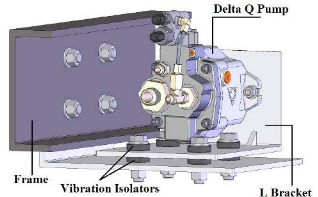
Figure 8: Pump Mounting L-Bracket Rear View
