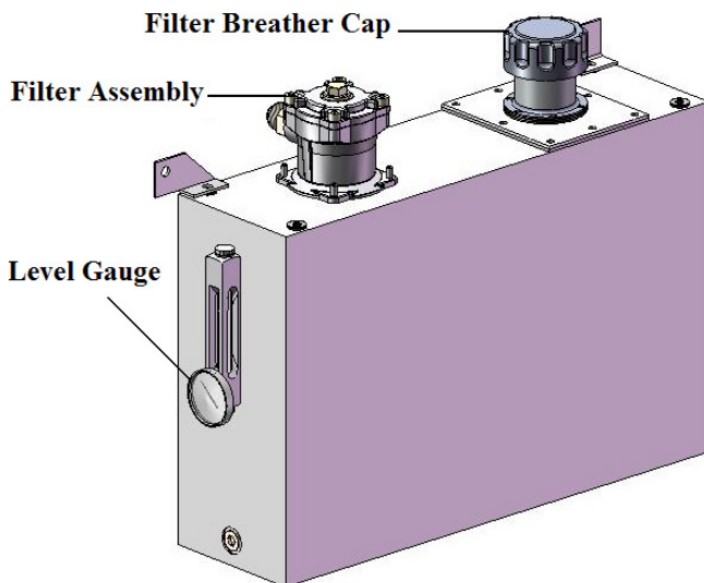
Figure 19: Hydraulic Fluid Reservoir
