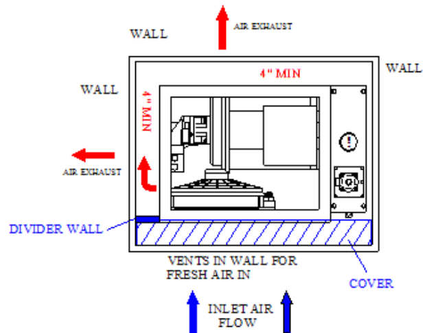
Figure 10: Generator Airflow
