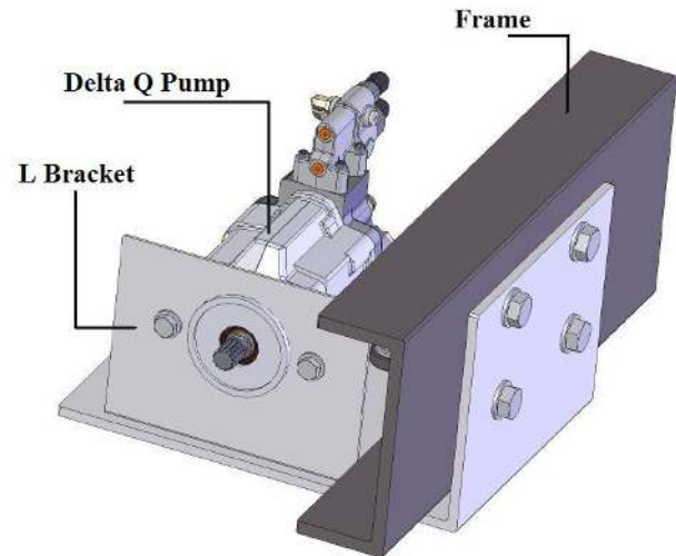
Figure 7: Pump Mounting L-Bracket Front View
