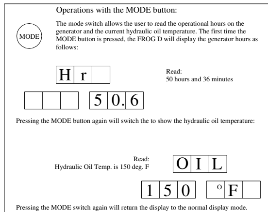
Figure 22: Display Mode Button
