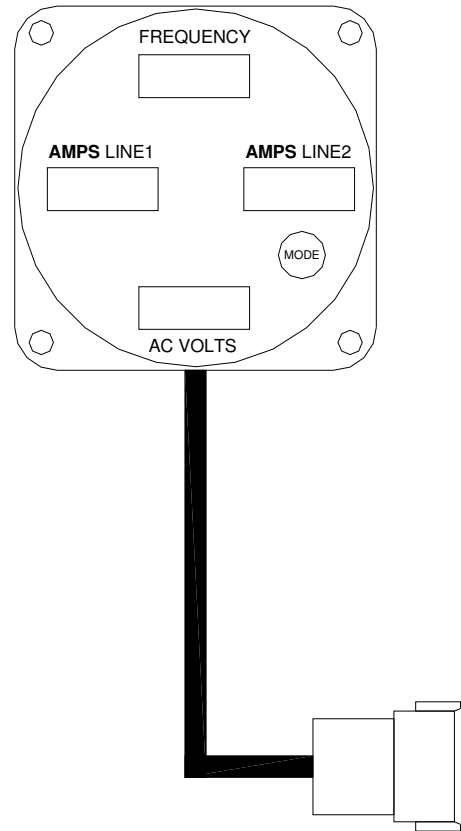
Figure 15: Display Meter
