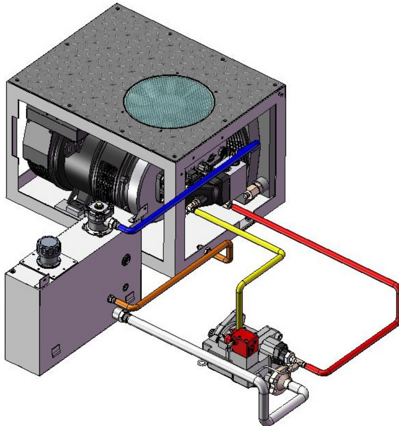
Figure 12: Detached Reservoir
