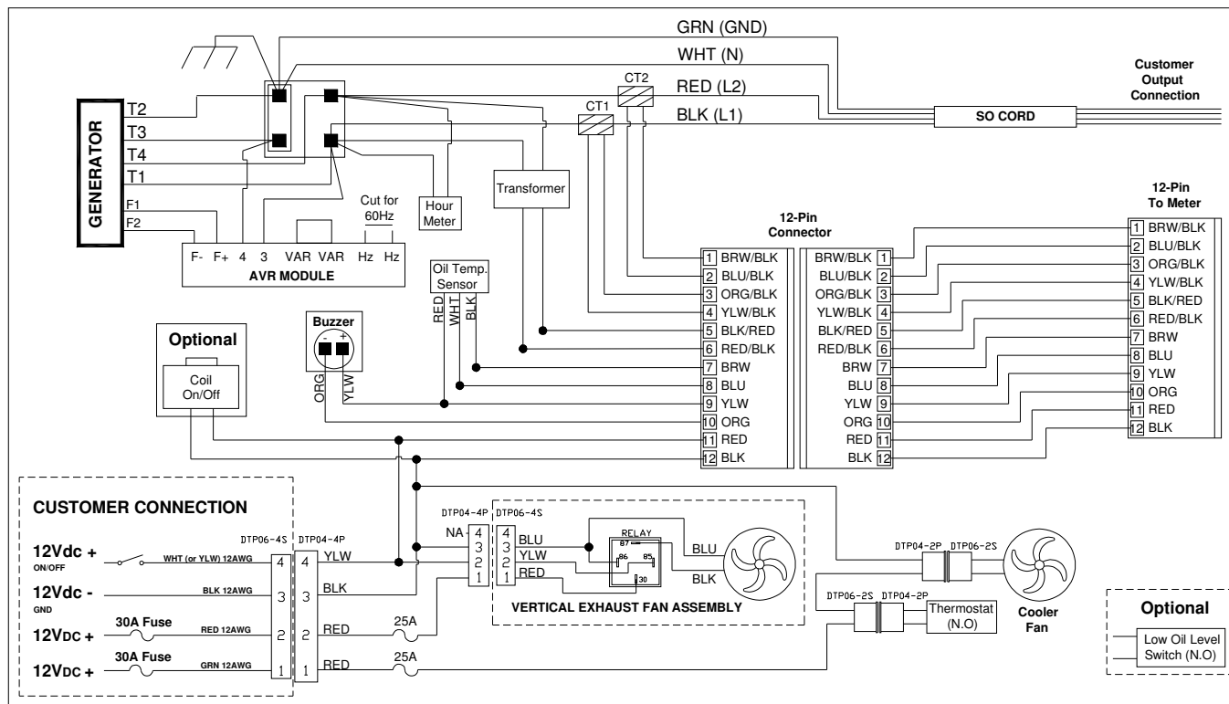
Figure 17: 10-20KW MPC Electrical Circuit Diagram for 120/240 1ph
