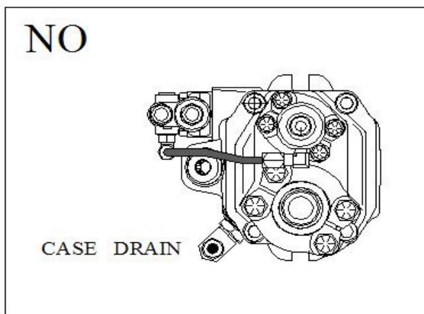
Figure 9: Pump Case Drain Orientation
