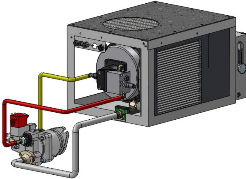
Figure 11: Attached Reservoir
