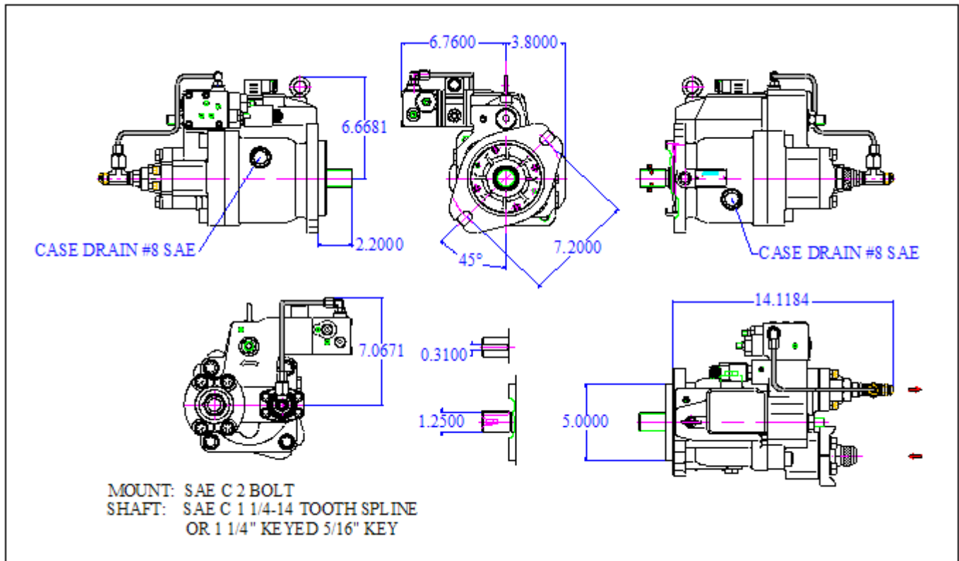
Figure 4: Kawasaki Pump Dimension
