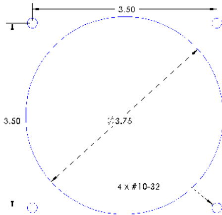
Figure 14: Display Meter Cutout Dimension
